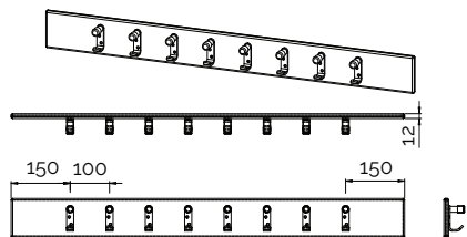
Our Hooks and Peg Boards available in different colours and materials
